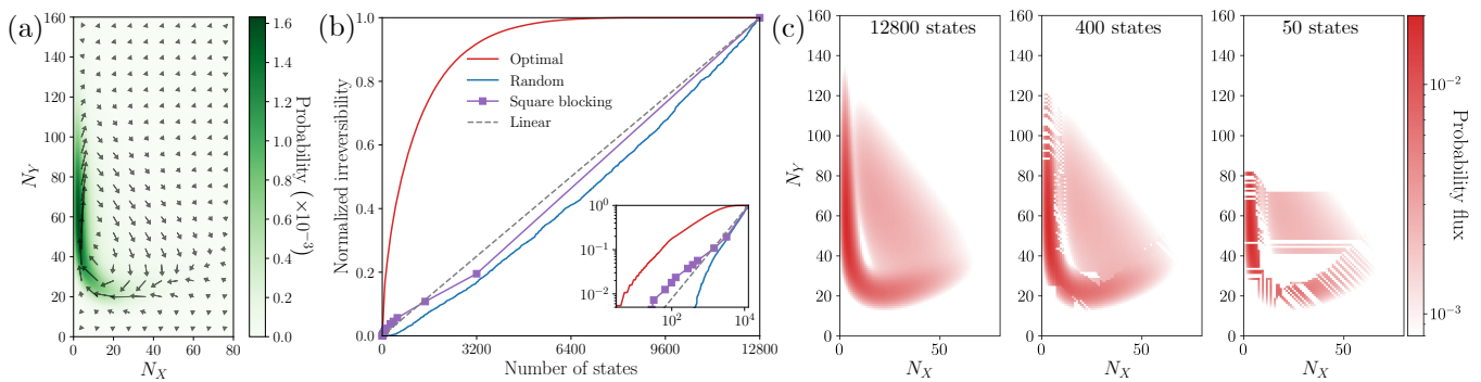
FIG. 2. Coarse-graining biochemical oscillations. (a) Steady-state probability density (colors) and net fluxes (arrows) in the Brusselator model of biochemical oscillations [43, 44]. Fluxes are averaged over local neighborhoods. (b) Fraction of irreversibility preserved after coarse-graining for three different procedures: optimal (red), random (blue), and square blocking (purple). Inset displays the same data on log-log axes. (c) Net fluxes between states in the full system with N = 12800 states (left) and under optimal CGs with 400 (center) and 50 (right) macrostates. Within each macrostate, fluxes are lost due to coarse-graining. See SM for details and parameters.
