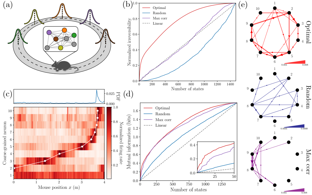
FIG. 3. Coarse-graining neural activity in the hippocampus. (a) A mouse runs along a one-dimensional virtual track as the activities of N = 1485 neurons are recorded in the hippocampus [46]. Approximately 30% of the neurons are place cells (indicated by colors in the neural network), which fire preferentially at specific locations along the track (indicated by location-dependent firing rates known as place fields). Mouse graphic adapted from Ref. [47] (CC BY 4.0). (b) Fraction of irreversibility preserved after coarse-graining for three different procedures: optimal (red), random (blue), and combining maximally correlated neurons (purple). (c) Place fields of 10 macrostates computed using the optimal CG with white points indicating the peaks. Top inset represents the distribution of mouse positions along the track. (d) Mutual information between coarse-grained neural activity and mouse position for different CG procedures. Inset is a zoomed-in view for the coarsest scales. (e) Probability flux between 10 macrostates. Note that the scale for random is 10 times smaller than optimal and max-corr.
