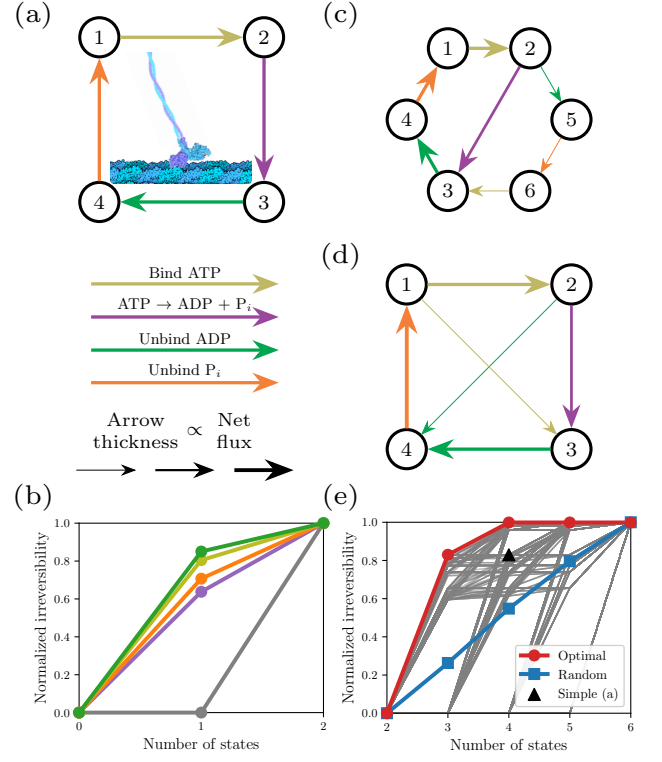
FIG. 1. Coarse-graining the kinesin chemical reaction cycle. (a) Minimal four-state model of the reaction cycle as the motor steps along the microtubule [39]. Colors and thicknesses of arrows represent the types and strengths of net fluxes [same for (c–d)]. Inset image adapted from PDB [40, 41]. (b) Fraction of irreversibility preserved under coarse-graining for the four-state model. Colors correspond to coarse-graining the different steps in (a); grey curves correspond to diagonal mergers (combining states 1 and 3 or 2 and 4), which destroy the irreversibility. (c) Six-state model with separate cycles for forward and backward steps [42]. (d) Optimal four-state CG of the six-state model. (e) Fraction of irreversibility preserved under coarse-graining for the six-state model. Grey curves show all possible CGs, red is optimal, blue is random (averaging over all CGs), and black is the four-state model in (a). See SM for details and parameters.
