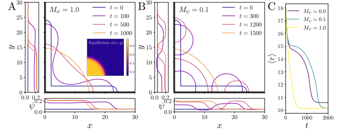
FIG. 2. (A–B) Dynamics of condensate localization for tether mobility M_\psi = 1.0 (A) and M_\psi = 0.1 (B). The simulation domain is a 2D system (x, y) with membranes on the left and bottom boundaries (indicated by thick black lines). Different colors indicate concentration profiles at different times (legend), with the condensate \phi represented by interface contours and the tether \psi shown in the left and bottom insets. Inset in (A) shows the final equilibrium profile for \phi(x, y) . The tether density at the boundaries is \psi_g = 0.05 . The overall \langle\phi\rangle is conserved due to no-flux boundary conditions. (C) Condensate location as quantified by the average distance \langle r \rangle = \int \delta\phi(x, y) \sqrt{x^2 + y^2} dx dy / \int \delta\phi(x, y) dx dy , where \delta\phi = \phi - \phi_g . See SI Appendix for details.
